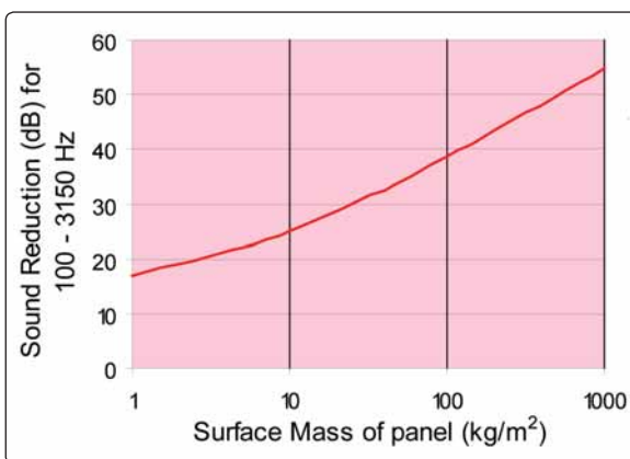
Figure 1 right: Mass Law Curve.
